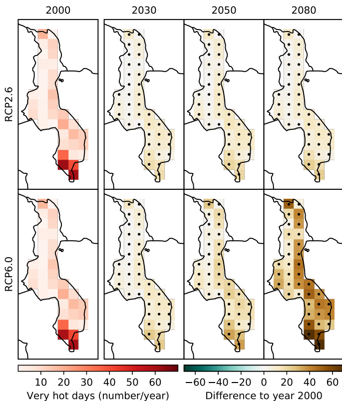
Figure 4: Projections of the number of very hot days (days with a maximum temperature >35 °C) per year for Malawi. The left-most column displays historical values for the year 2000, the other columns display projections for the years 2030, 2050 and 2080. The upper row shows projections under RCP2.6, the lower row those under RCP6.0. A dot in a grid cell indicates high agreement between the models and thus low uncertainty.
