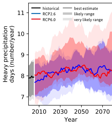
Figure 6: Projections of the number of days with heavy precipitation in Malawi under different GHG emissions scenarios, relative to the year 2000.
