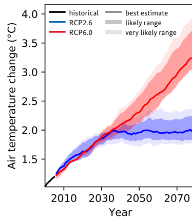
Figure 3: Projected changes in air temperature relative to 1876 for Malawi for different GHG emissions scenarios.
