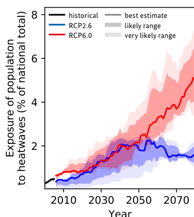
Figure 18: Projected share of the population exposed to humid heatwaves at least once per year for Malawi under different GHG emissions scenarios.
