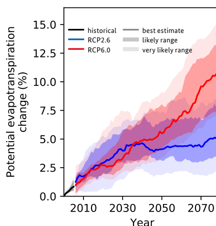
Figure 8: Projected changes in potential evapotranspiration for Malawi for different GHG emissions scenarios, relative to the year 2000.
