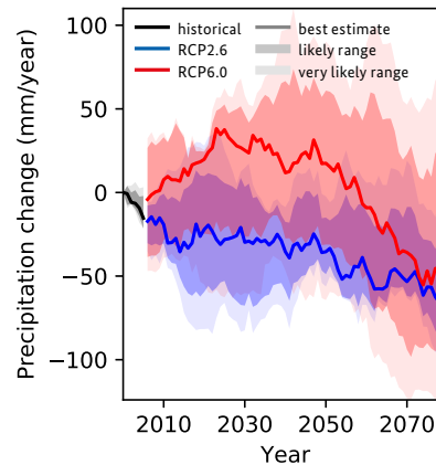
Figure 5: Projected changes in precipitation for Malawi in mm per year relative to the year 2000 for different GHG emissions scenarios.
