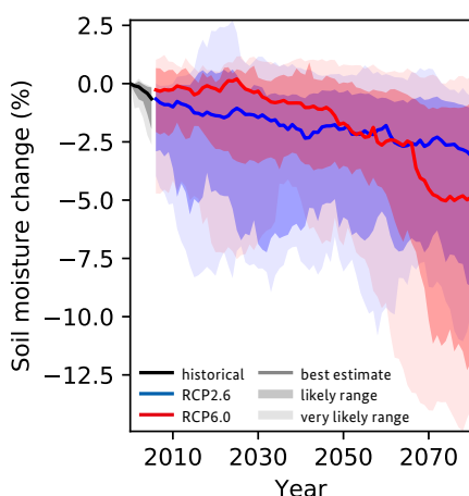
Figure 9: Projected changes in soil moisture for Malawi for different GHG emissions scenarios, relative to the year 2000.
